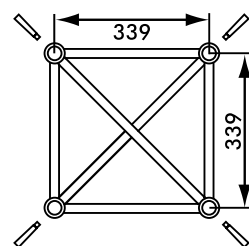
Figure 7 X40V dimensions
