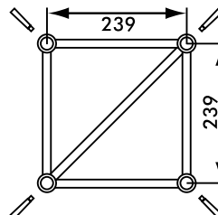
Figure 5 H30V dimensions
