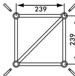
Figure 3 X30V dimensions
