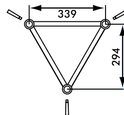
Figure 6 X40D dimensions
