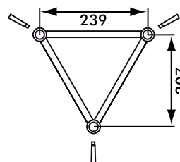
Figure 4 H30D dimensions
