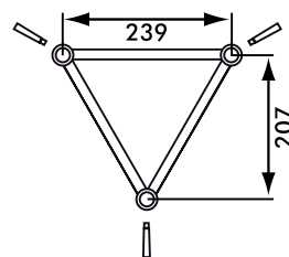
Figure 2 X30D dimensions
