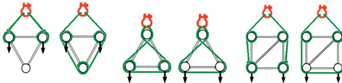
Figure 13 Approved slinging methods
