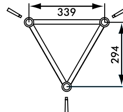
Figure 8 H40D dimensions
