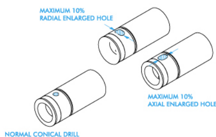
Figure 18 Oval-shaped holes
